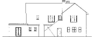
Proposed North Elevation
