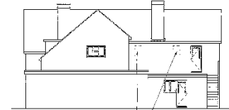
Proposed East Elevation
